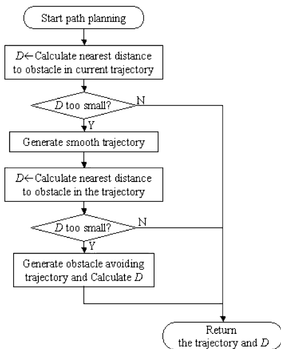
Fig. 16. Generic real-time path adjustment.
